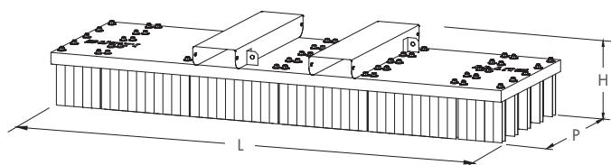
QUOTE SEDI FORCHE FORK SEATS DIMENSIONS
